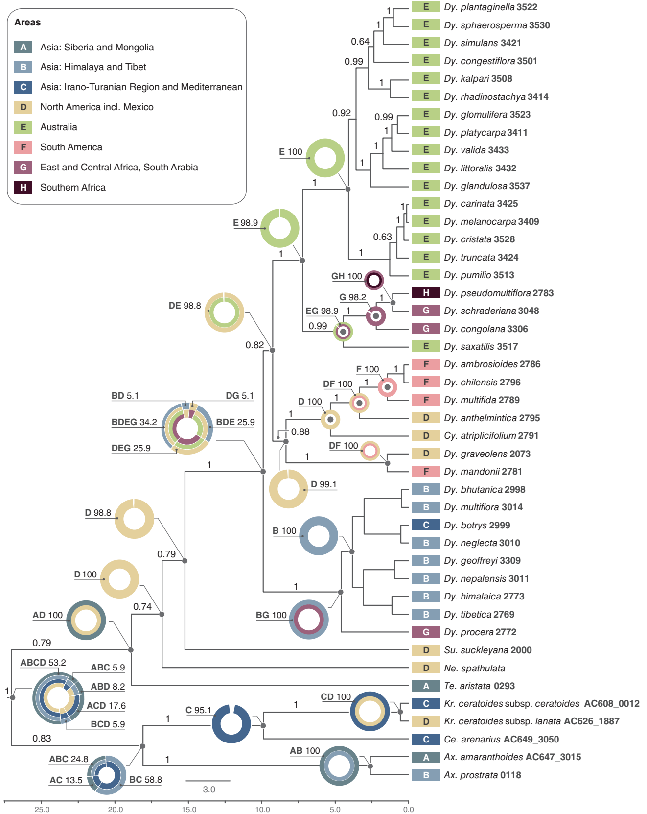
Fig. 4. Results of the ancestral range estimation (ARE) under the DIVALIKE model and with a maximum of four ancestral areas allowed, run with BioGeoBEARS based on a time-calibrated tree representing 44 species and subspecies of Dysphanieae with only one accession per species. Numbers above branches represent posterior probabilities.
